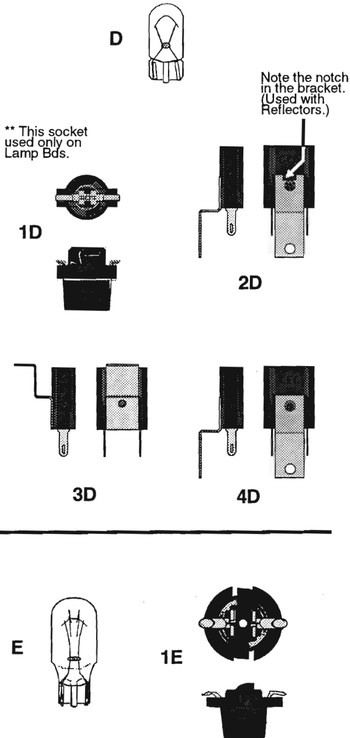
UNDER PLAYFIELD: BOTTOM VIEW
