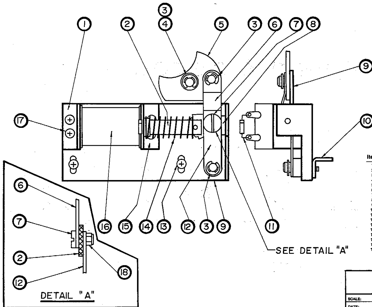
500-5104-00 LOCK BALL BRACKET ASSEMBLY
