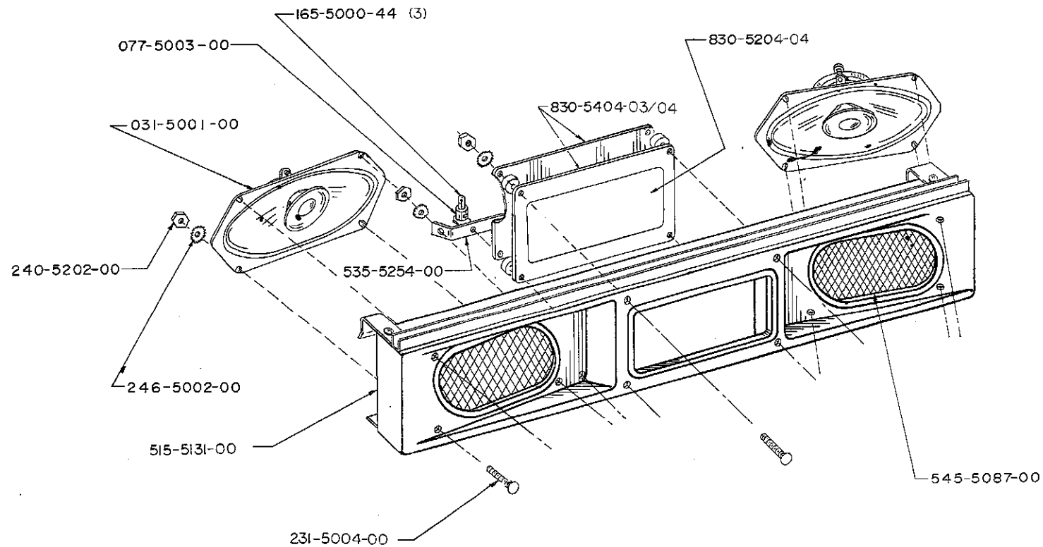
500-5124-00 SPEAKER HOUSING ASSEMBLY
