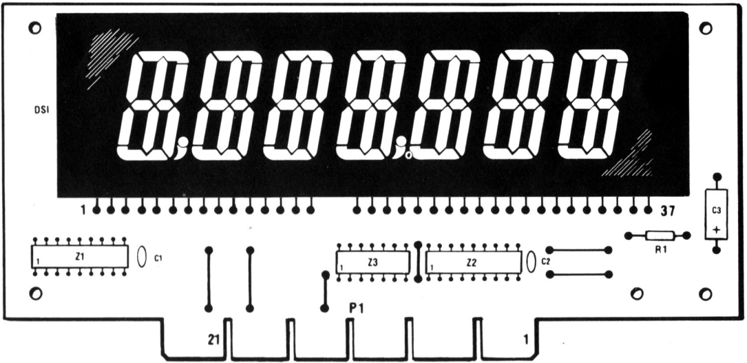
7-DIGIT DISPLAY (A14) PARTS LIST
