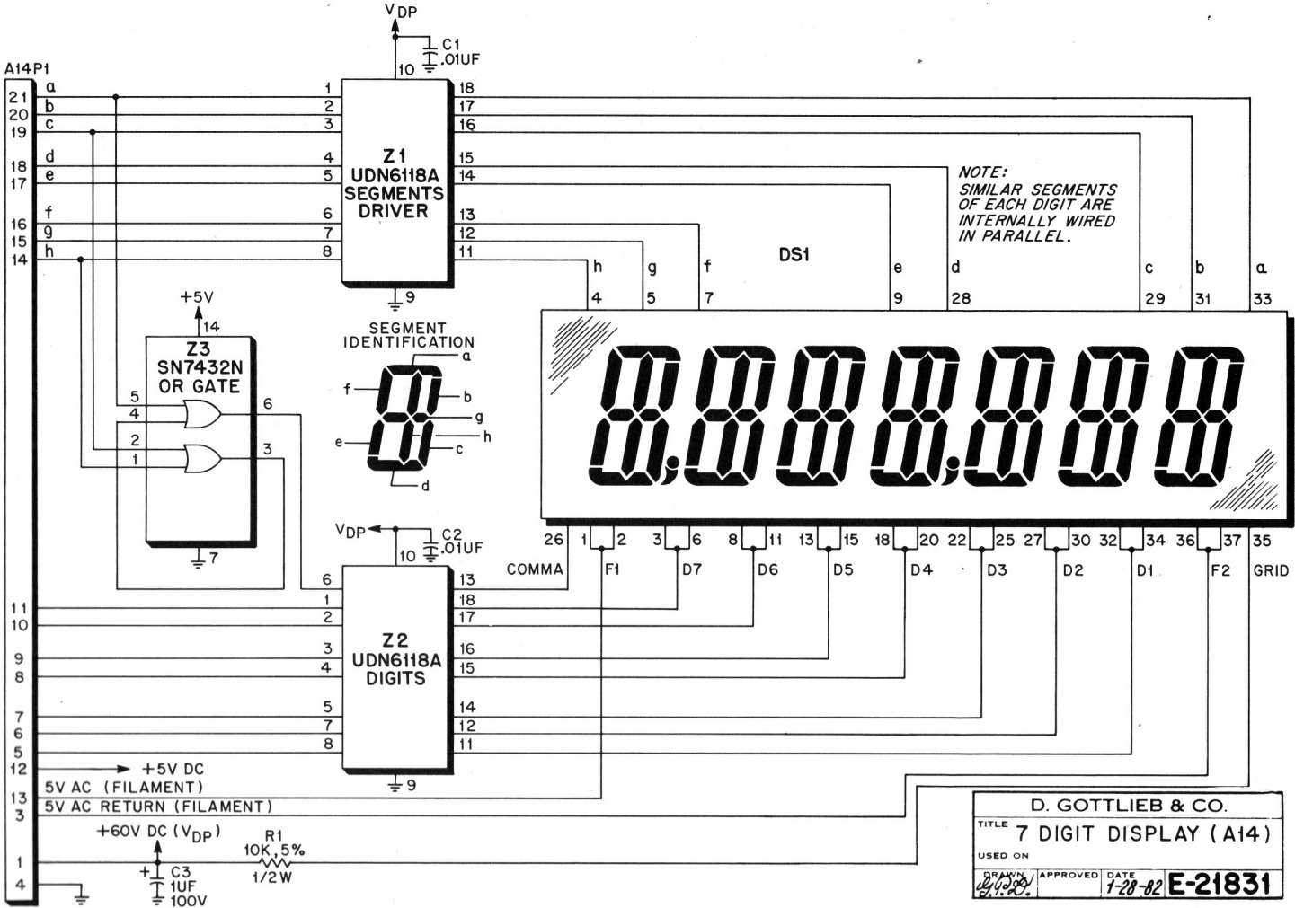
7-DIGIT DISPLAY (A14) COMPONENT LOCATION
