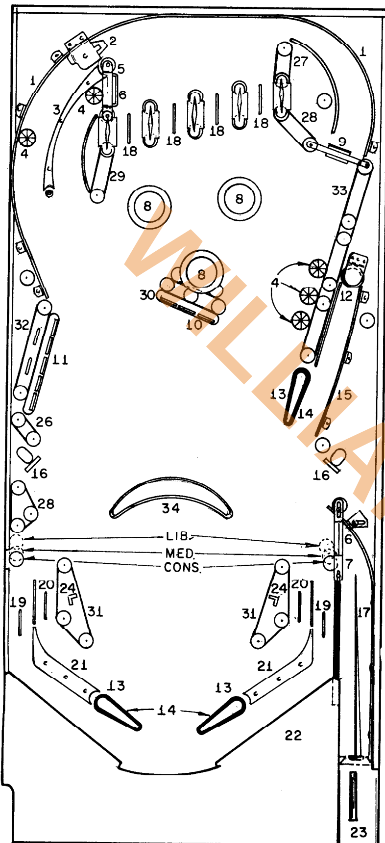
Figure 14. Playfield Spare Parts
