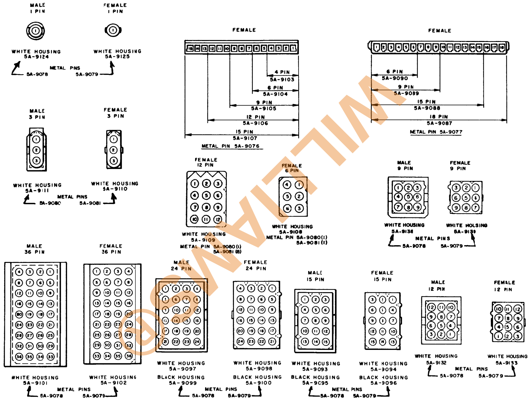
Figure 13. Connector Details
