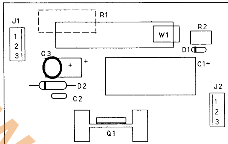
Board Assembly
