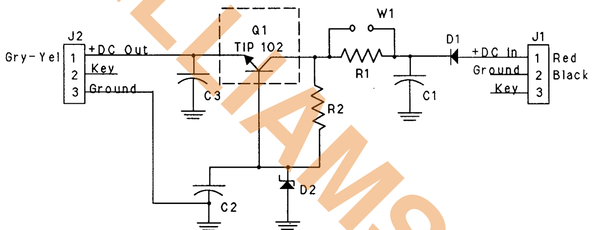
Schematic
