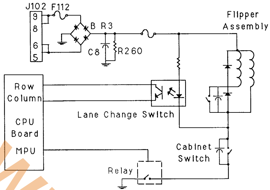
Wiring Diagram
